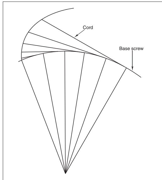
Figure 8-3: Involute form is generated by unwrapping a cord from a circle
